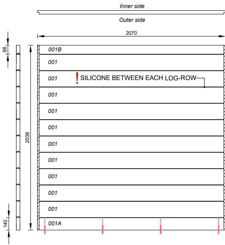
WALL B (BACK) VIEW FROM THE OUTSIDE
